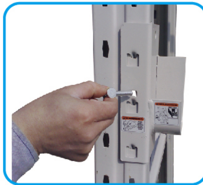
Safety Pin Locks Axle Bracket
